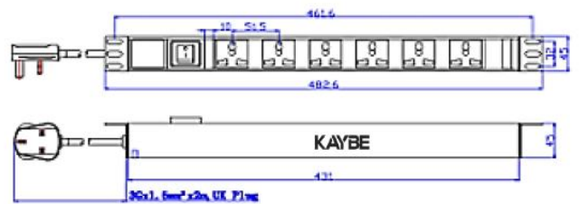
Schematics drawings
