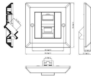
Schematics drawings
